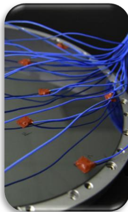
E-Chuck Heater Electrode
